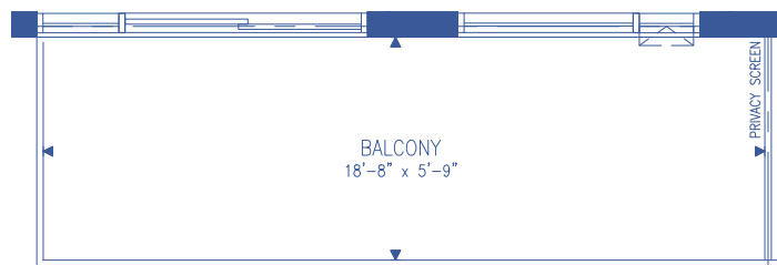
BALCONY AT LEVEL 2 TO LEVEL 10 - SUITE 30
